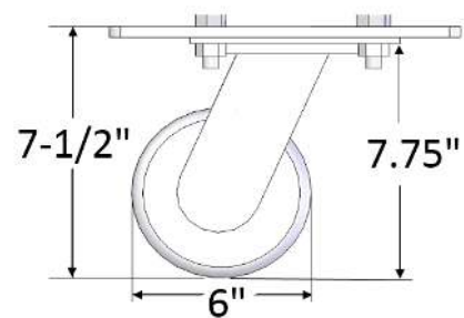
PN #48-979013 Skid Wheel 6" Class A
